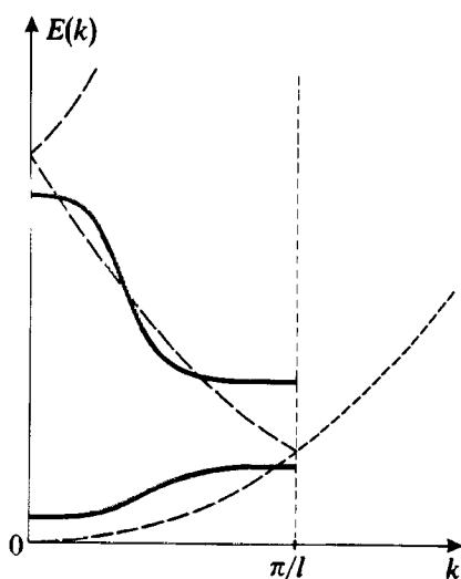
FIGURE 6 Variation of the energy with respect to the parameter k . The solid lines correspond to the energies for the first two allowed bands (the values of k which give the energy levels being equidistant inside the interval 0 \leq k \leq \pi/l ). The dashed lines correspond to the special case where the potential V(x) is zero (a free particle); the allowed bands are contiguous, and there are no forbidden bands.
